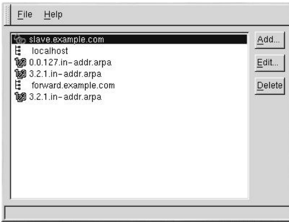
Figure 15-1. bindconf
