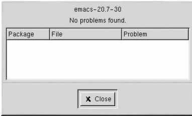
Figure 26-10. Verify Window
