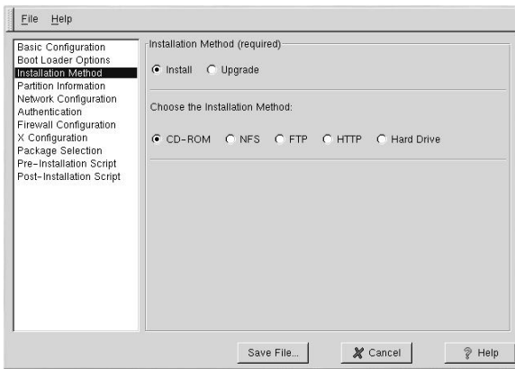
Figure 2-3. Installation Method
