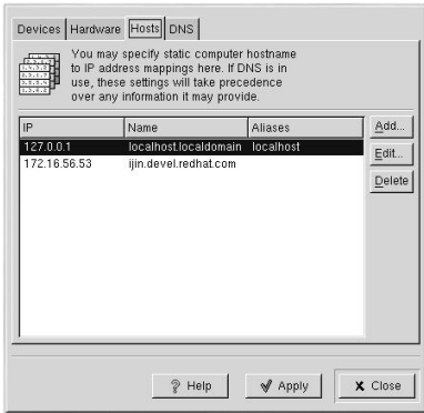
Figure 6-14. Hosts Configuration
