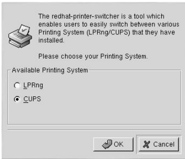
Figure 21-17. redhat-switch-printer
