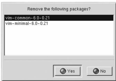
Figure 26-11. Uninstall Window
