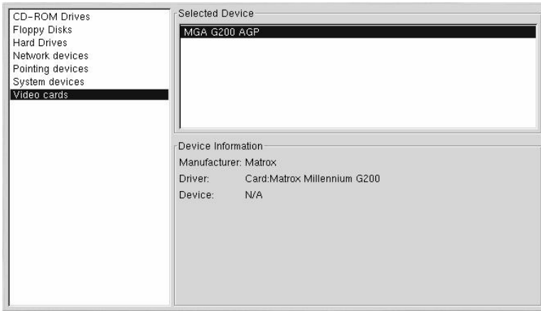
Figure 20-4. Hardware Browser
