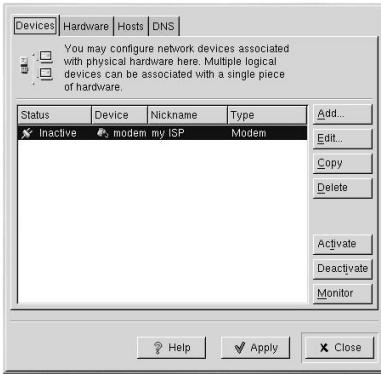
Figure 6-6. Modem Device
