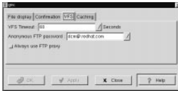
Figure 6-9. VFS Preferences
