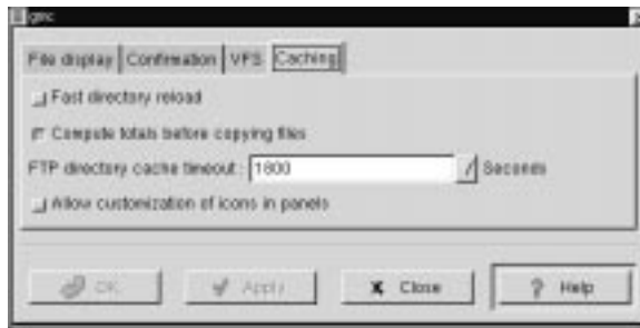
Figure 6-10. Caching Preferences
