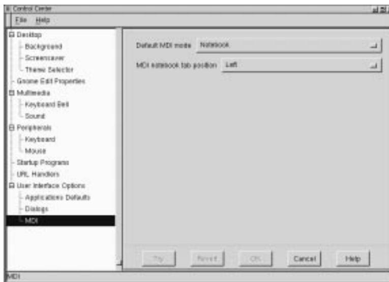
Figure 9-16. MDI Cappellet
