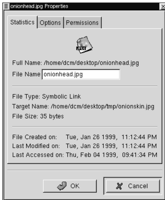
Figure 6-6. File Properties
