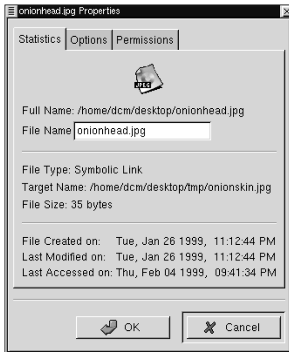
Figure 6-4. File Properties
