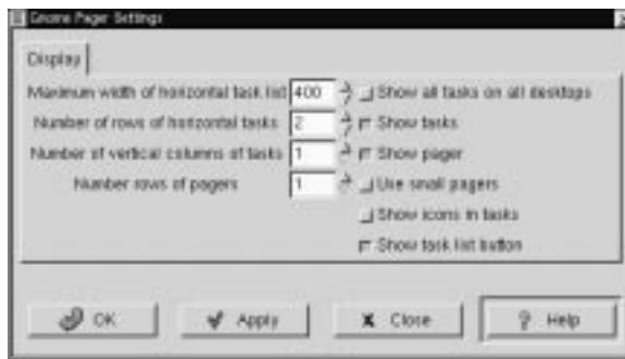
Figure 11-11. The GNOME Pager Properties
