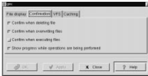
Figure 6-8. Confirmation Preferences
