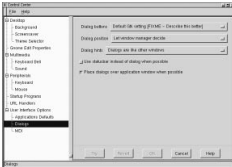
Figure 9-15. Dialog Capplet
