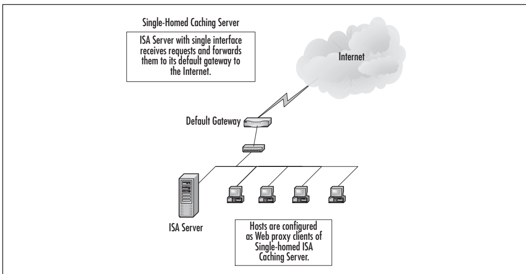
Figure 4.3 A Single-Homed Web-Caching-Only Server
