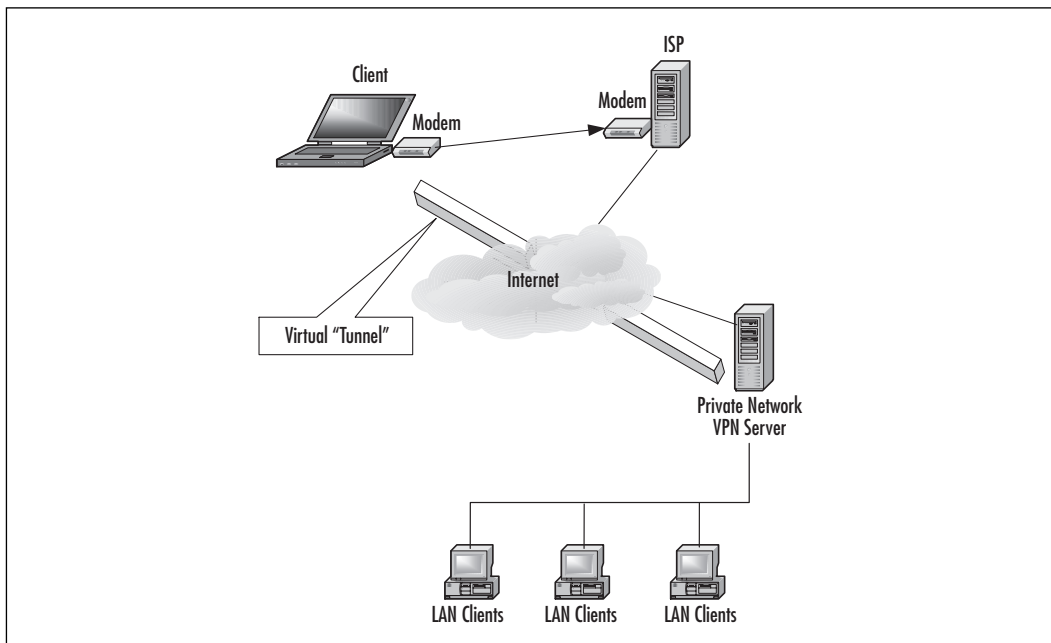
Figure 1.9 A VPN Allows Establishment of a Secure Link to a Private Network Across the Public Internet
