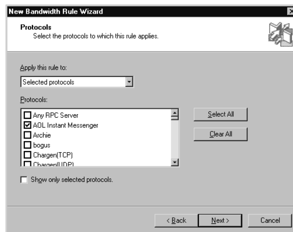
Figure 8.38 Choosing Protocols
