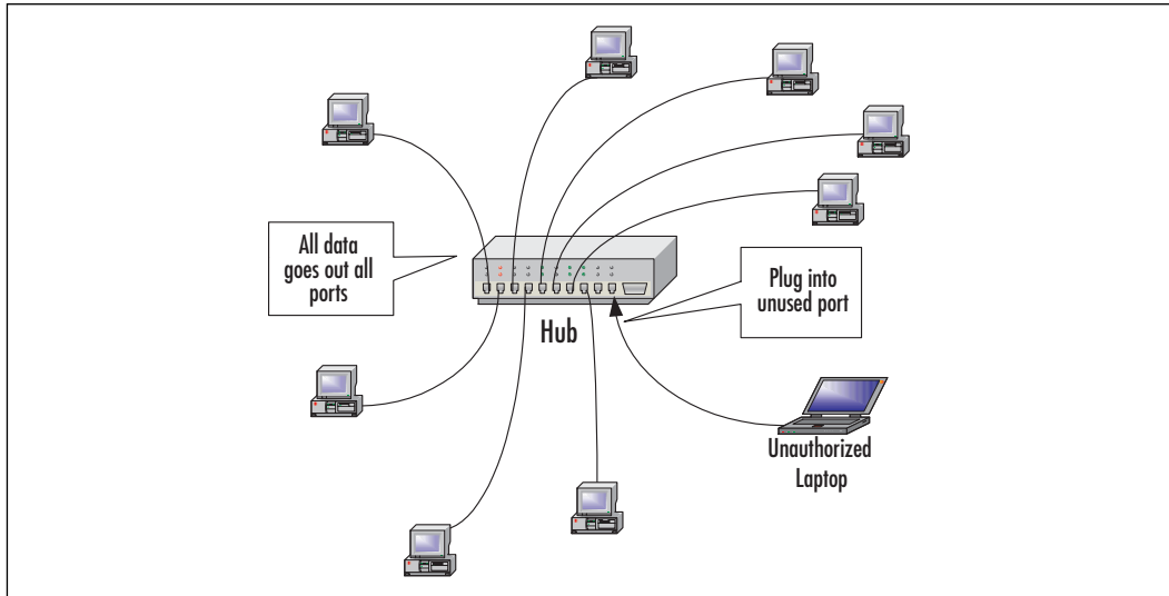
Figure 3.2 An Intruder with Access to the Hub Can Easily Intercept Data
