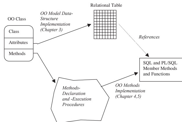
Figure 5.1. Generic methods
