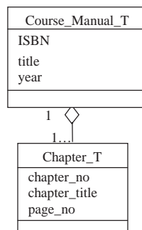
Figure 5.19. Aggregation relationship
