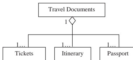
Figure 1.10. Existence-independent composition
