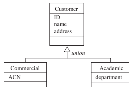
Figure 5.2. Union inheritance
