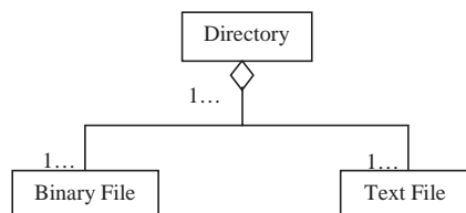
Figure 1.12. Nonexclusive composition
