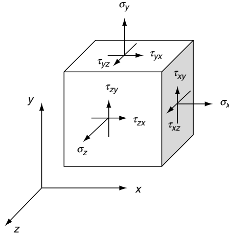
FIGURE 3-3 Components of the stress.
