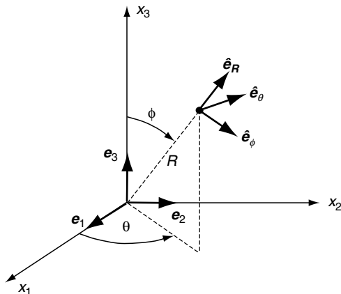
FIGURE 1-5 Spherical coordinate system.
