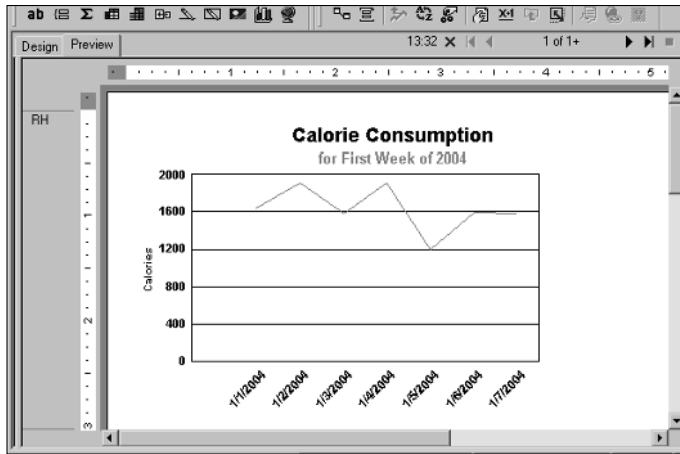
Figure 15-4: Line chart.
