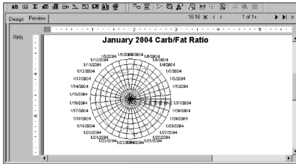
Figure 15-11: Radar chart.
