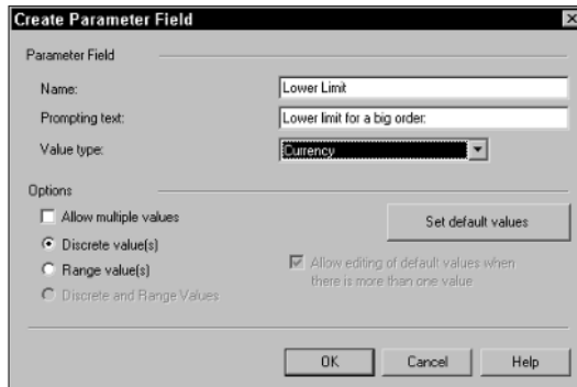
Figure 5-16: Create Parameter Field dialog box, speci- fying the lower limit parameter field.
