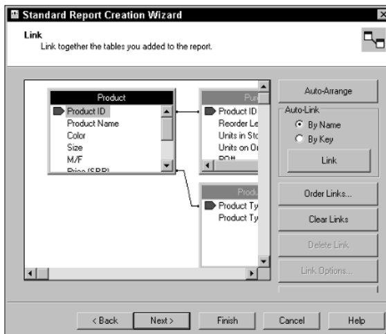
Figure 5-1: Selected tables and their rela- tionships.
