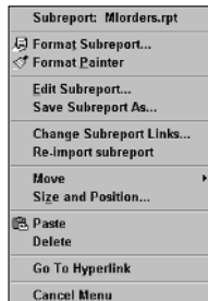
Figure 12-10: Subreport menu.
