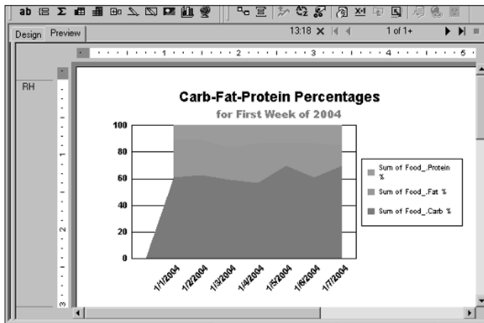
Figure 15-5: Area chart.
